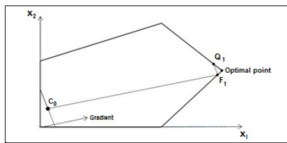
Figure 4. Orthogonal projection ( Q_1 )
